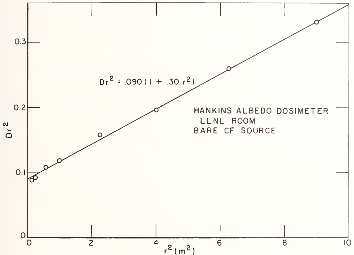
Figure 1 - Response of the Hankins Albedo Dosimeter per unit dose equivalent as a function of distance from the neutron source. The measurements were taken with a bare ^{252}\text{Cf} source in the LLNL calibration room. The data are fitted to an equation of the form
